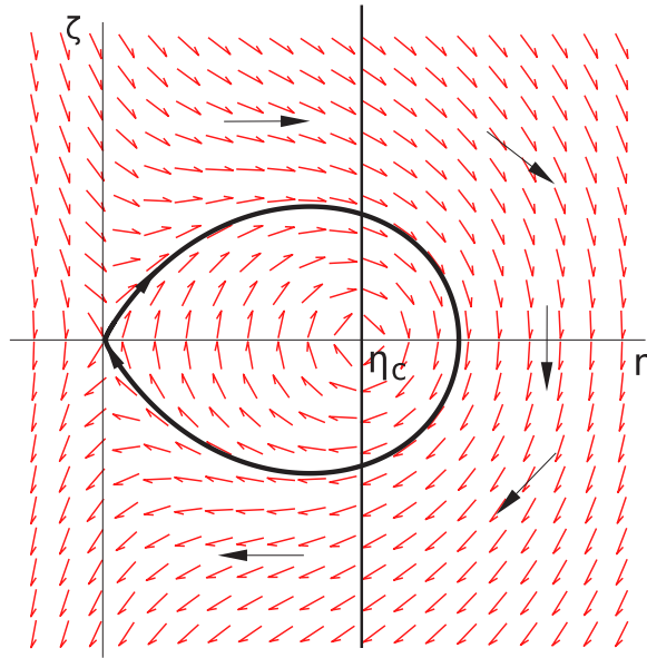
Fig. 2. Phase portrait of system (4.4) for c = 2 with a homoclinic orbit emerging from the origin which corresponds to a solitary wave solution of the equation for surface waves of moderate amplitude in the shallow water regime.
