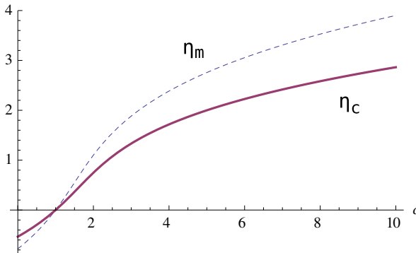
Fig. 3. The x -coordinate \eta_c of the critical point P_c = (\eta_c, 0) and the maximum height \eta_m of the wave profile as a function of the wave speed c .
