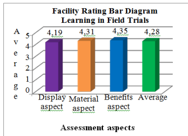
Fig. 1. Assessment aspects
